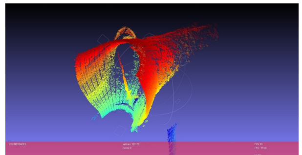
3D Sonar Point Data from Intake at Bifurcation
